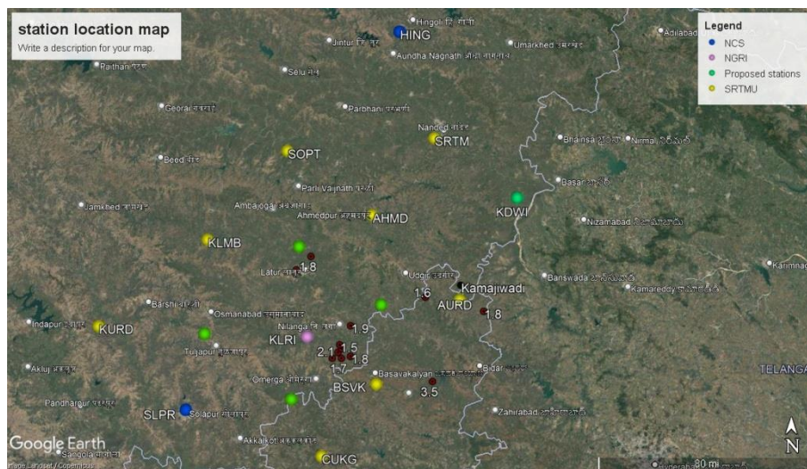
Image displaying 11 station grid around the intraplate earthquake source region Latur
